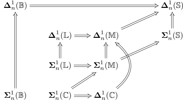
FIGURE 2. An incomplete diagram of implications for \Sigma_n^1 and \Delta_n^1 sets of reals.
