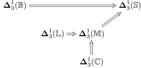
FIGURE 3. Diagram of implications for \Delta_3^1 sets of reals.
