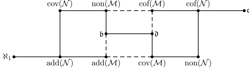
FIGURE 1. Cichoń's diagram
